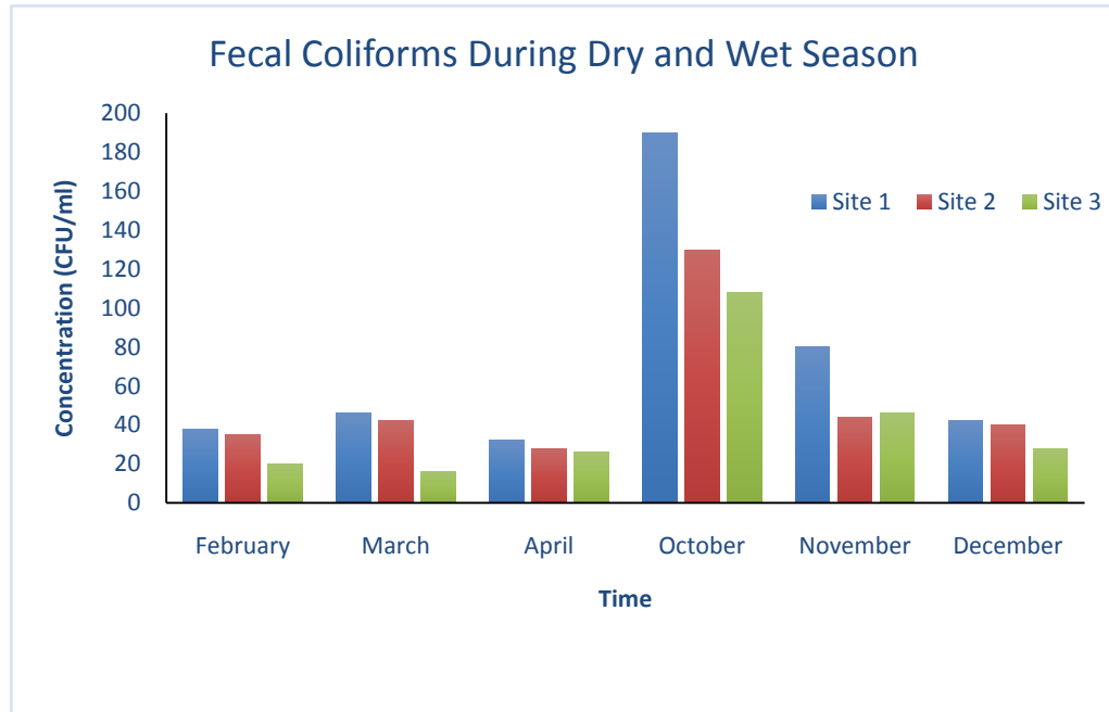
Figure 3. Concentration of Fecal Coliforms During Wet and Dry Season
