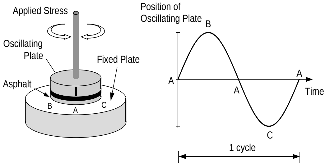
Figure 2. Operational mechanism of DSR test
