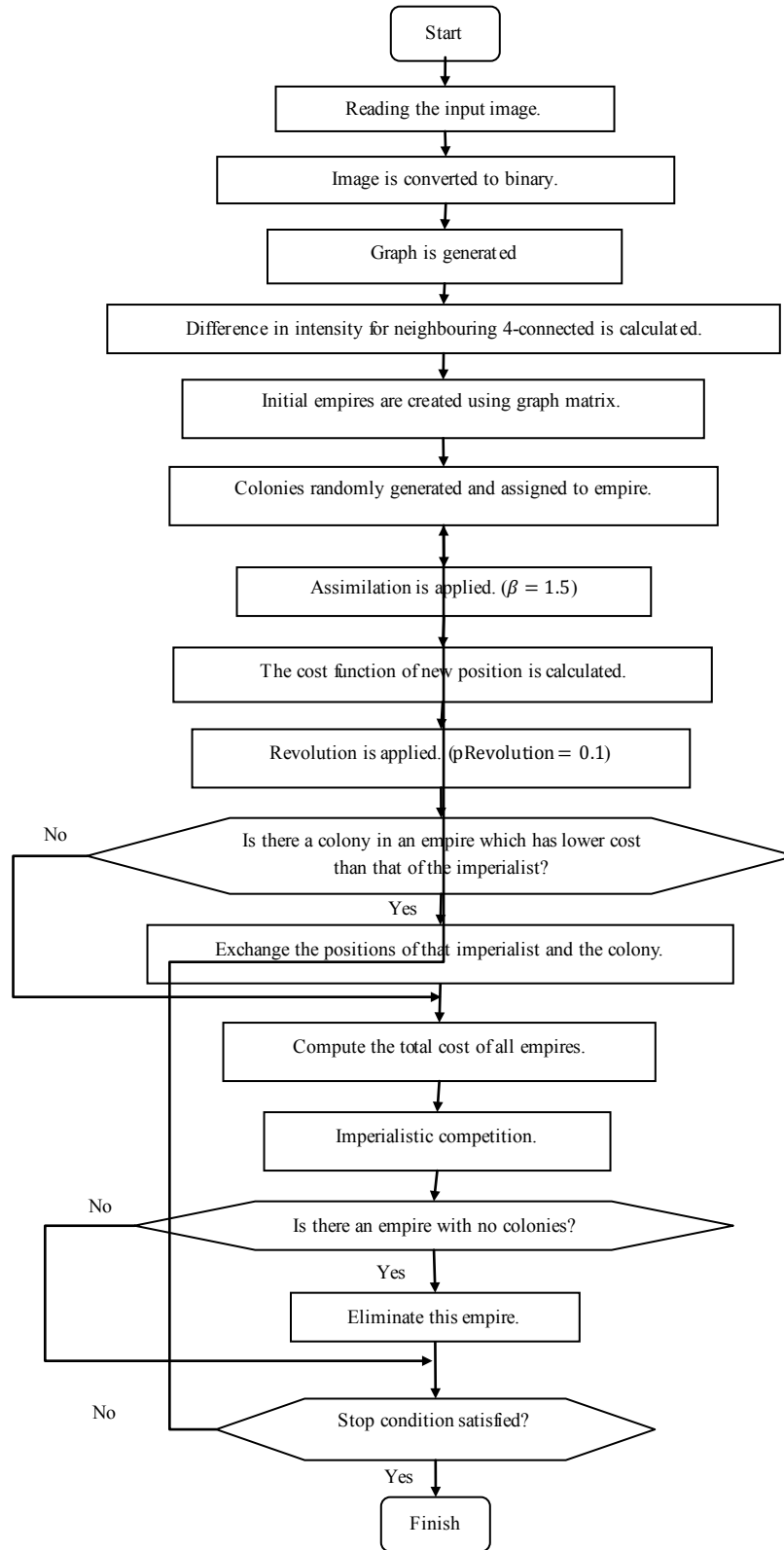
Figure 2. Flowchart of resolving the image segmentation problem by graph partitioning based on ICA
