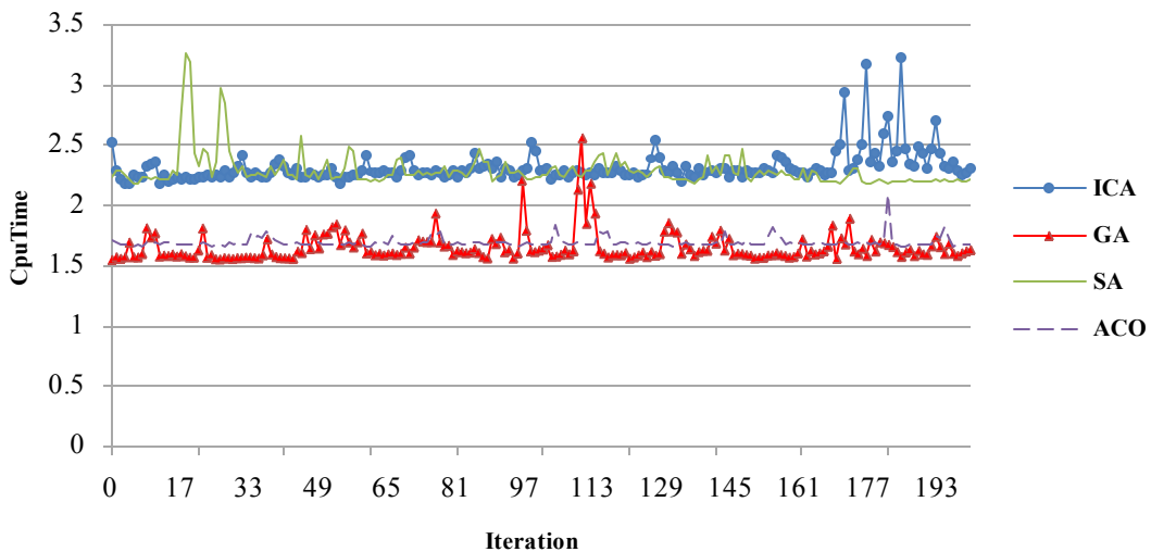
Figure 10. time required for each algorithm implementation
