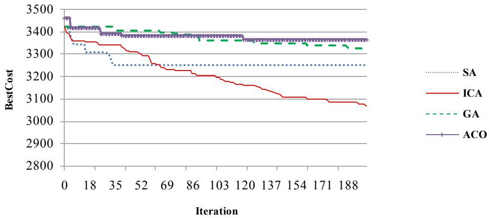
Figure 8. comparing the different algorithm to find the best answer of each generation of image 5
