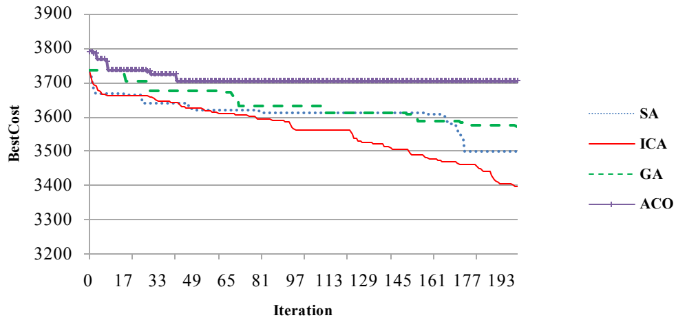
Figure 5. comparing the different algorithm to find the best answer of each generation of image 2
