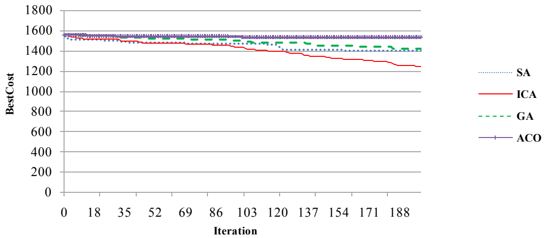
Figure 6. comparing the different algorithm to find the best answer of each generation of image 3
