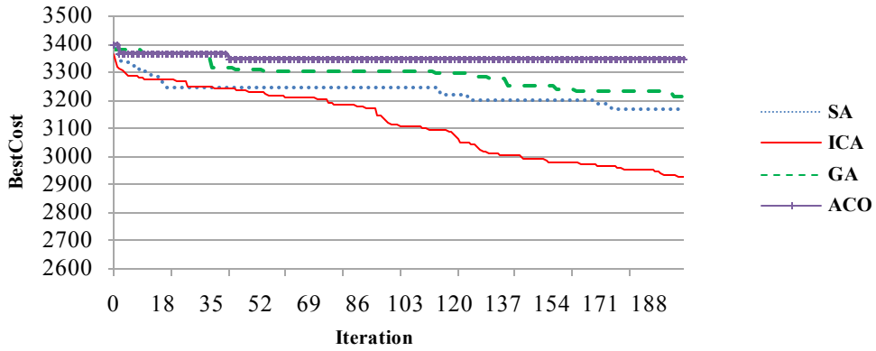
Figure 7. comparing the different algorithm to find the best answer of each generation of image 4
