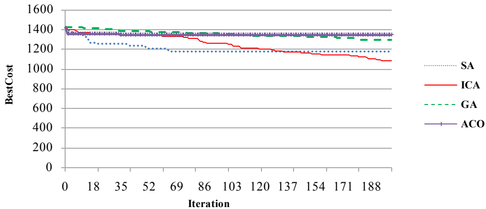
Figure 4. comparing the different algorithm to find the best answer of each generation of image 1
