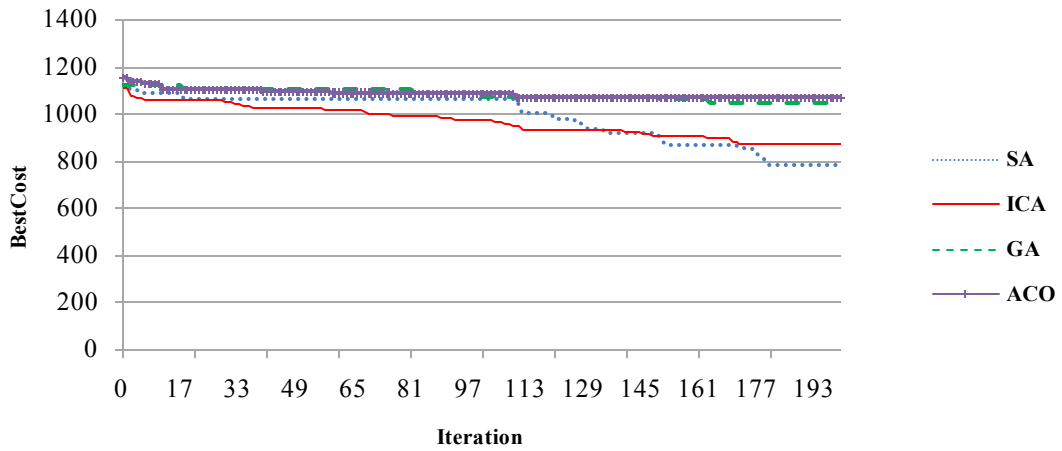
Figure 9. comparing the different algorithm to find the best answer of each generation of image 6
